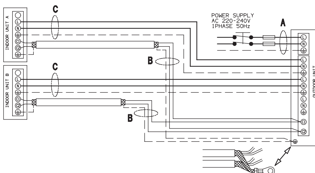
2 INDOOR UNITS
