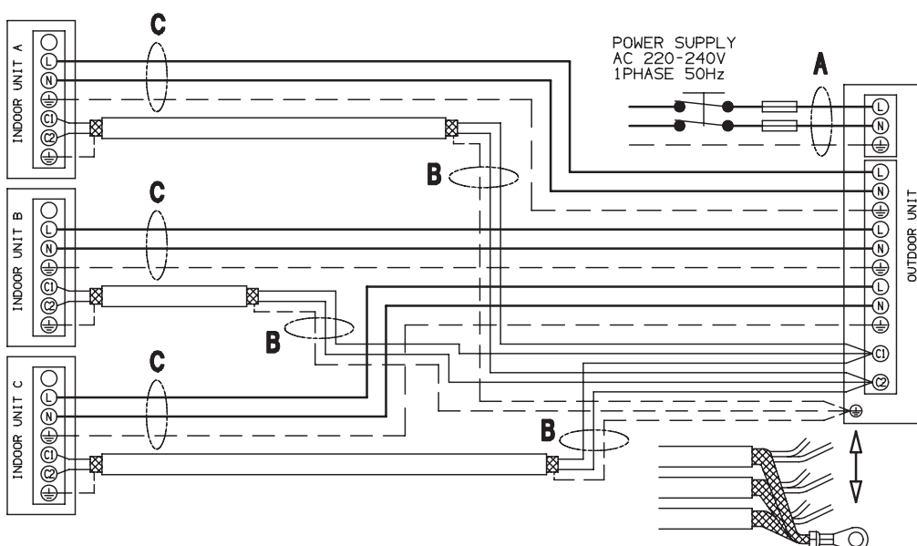
3 INDOOR UNITS
